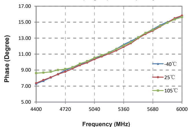
Phase (Degree) VS.Frequency
